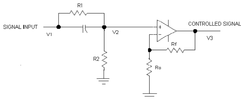
Fig.11) lead compensator
